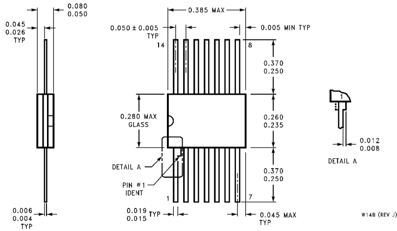
14-Lead Ceramic Flatpak (F) NS Package Number W148
